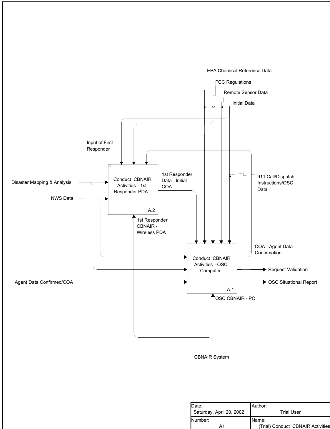
Figure #5 A1 Diagram Perform CBNAIR Activities
