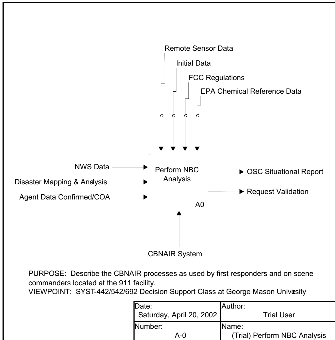
Figure #4 A-0 Diagram Perform NBC Analysis
